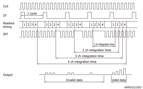
[Figure 8] Timing chart (variable integration time function)
