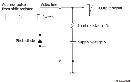
[Figure 11] Operation of current-to-voltage conversion method
