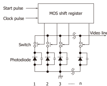
(a) NMOS linear image sensor (S3901 to S3904 series)
