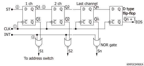
[Figure 5] Circuit of shift register with readout control function
