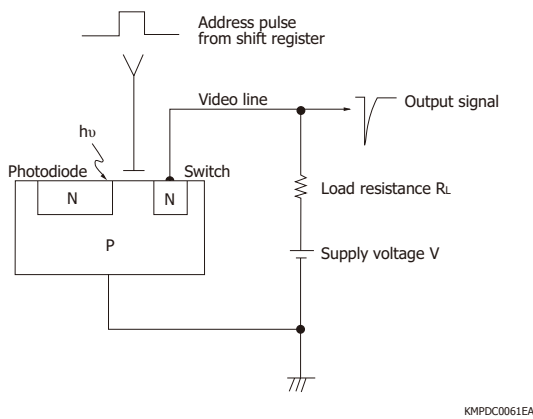
[Figure 10] Equivalent circuit of current-to-voltage conversion method
