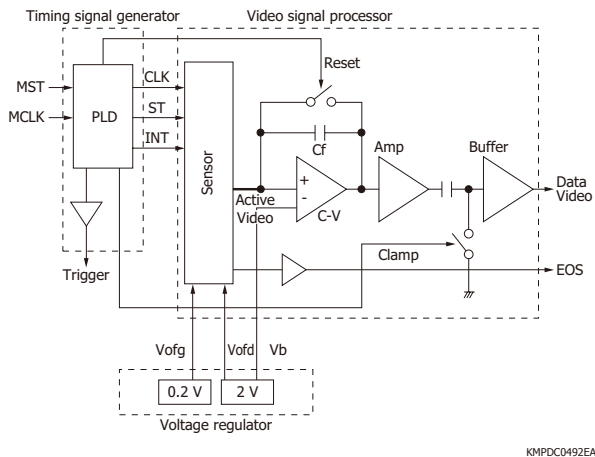
[Figure 12] External driver circuit example
