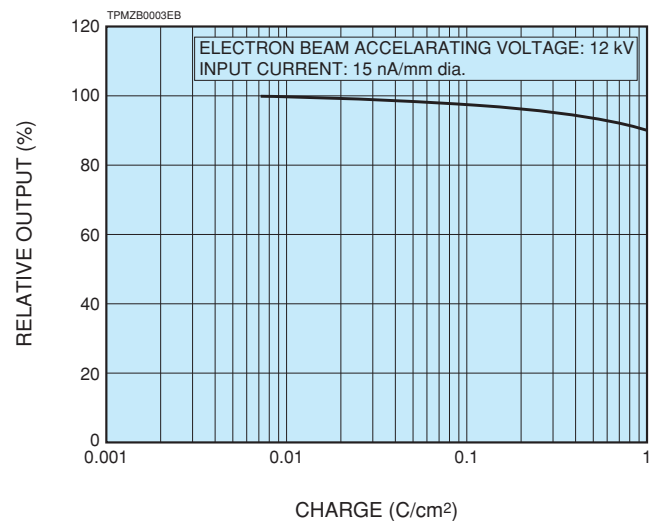
Figure 2: Life characteristics
