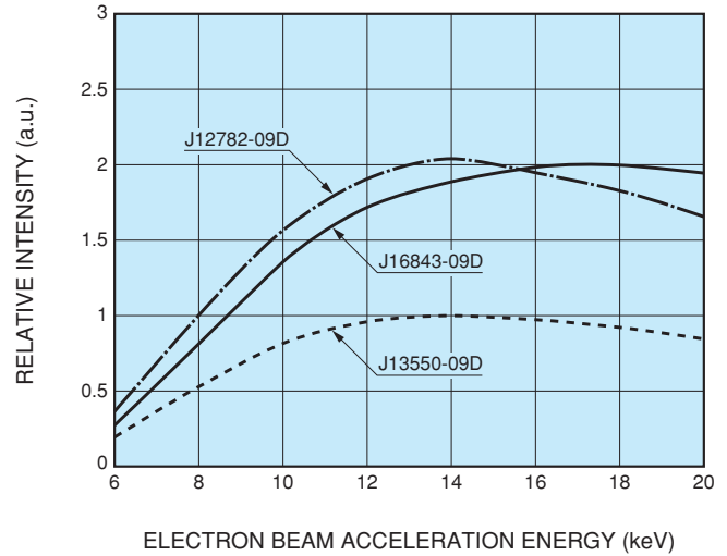
Figure 4: Relative light emission intensity (measurement data example)
