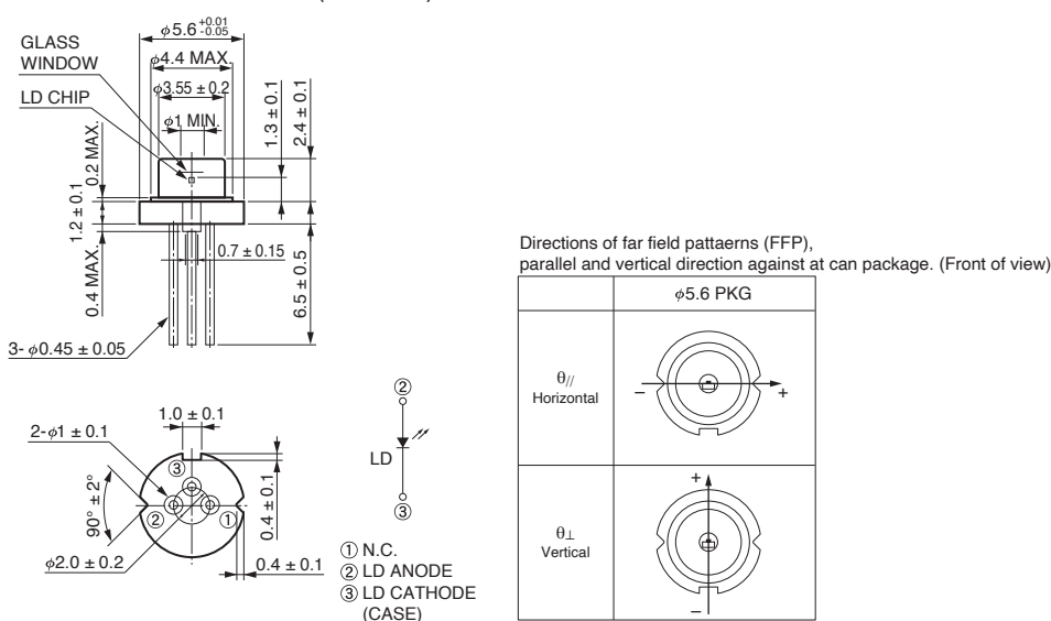
Figure 5: Dimensional outline (unit: mm)
