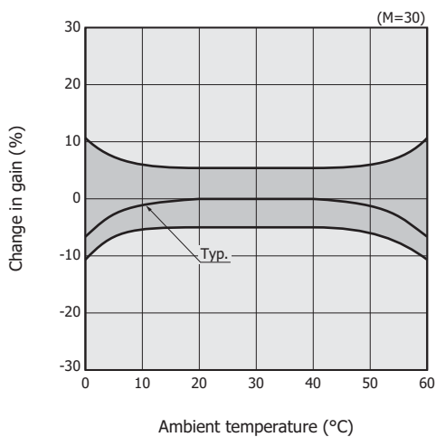
[Figure 5] Temperature characteristics of gain (C12703 series)
