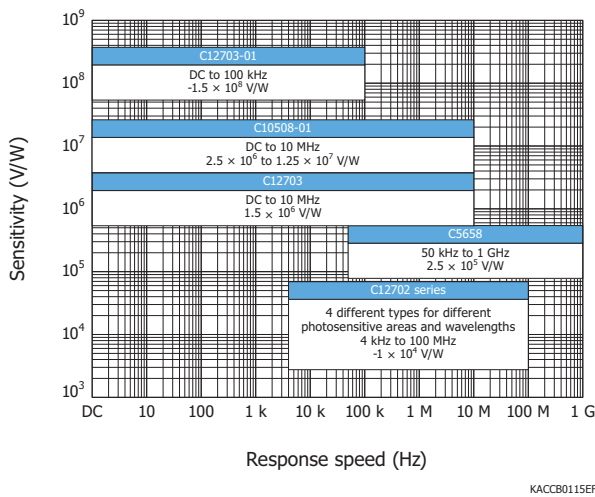
[Figure 1] Sensitivity vs. response speed
