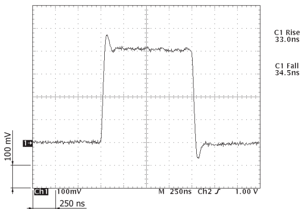
Ta=25 °C, gain=30, incident pulse width=1 \mu s X-axis: 250 ns/div, Y-axis: 100 mV/div.
