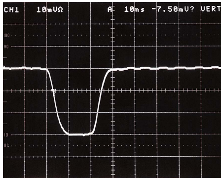
Ta=25 °C, gain=30, incident pulse width=20 ns X-axis: 10 ns/div, Y-axis: 10 mV/div.
