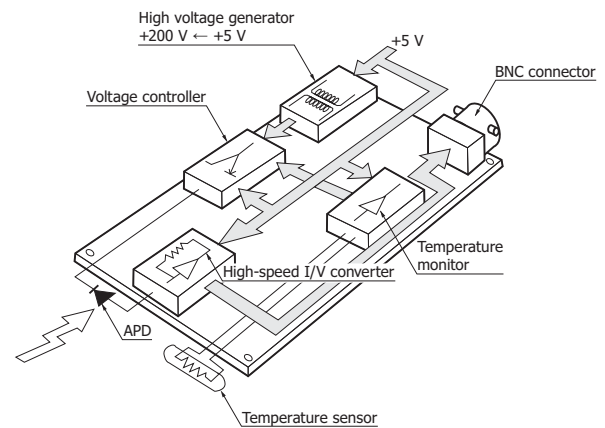
[Figure 2] Block diagram (C12702 series)
