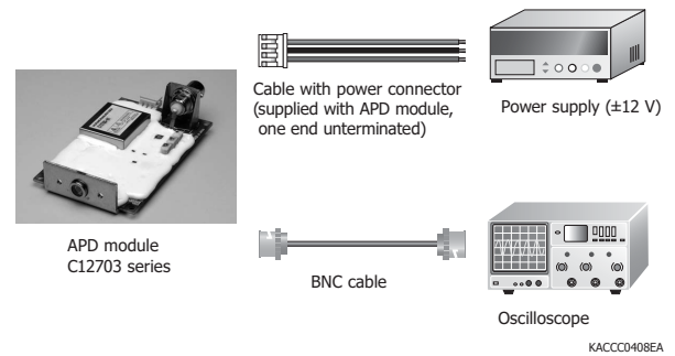
[Figure 6] Connection example (C12703 series)
