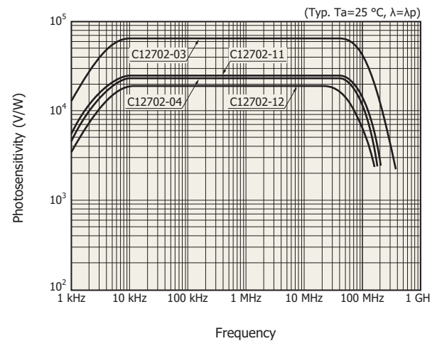
[Figure 3] Frequency characteristics
