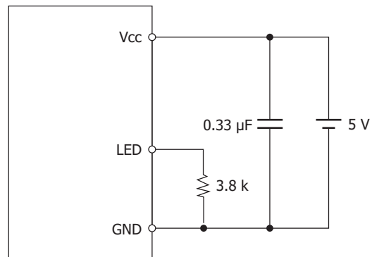
Measurement circuit
