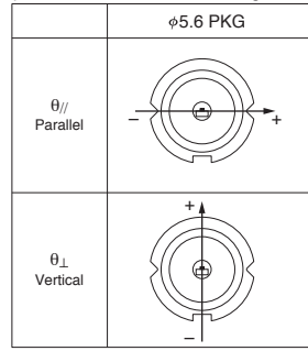
Directions of far field patterns (FFP), parallel and vertical direction against at can package. (Front of view)
