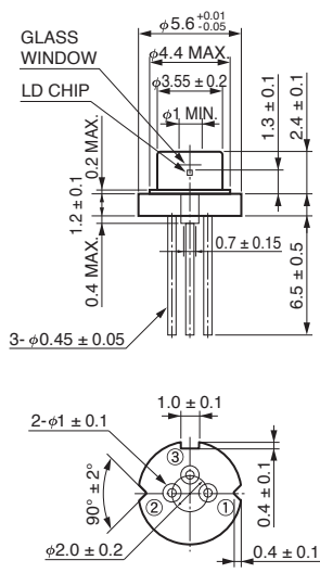
Figure 5: Dimensional outline (unit: mm)
