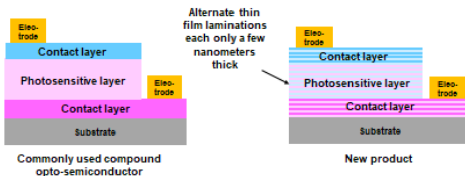
Different structures: common (left) and new (right) compound opto-semiconductors
