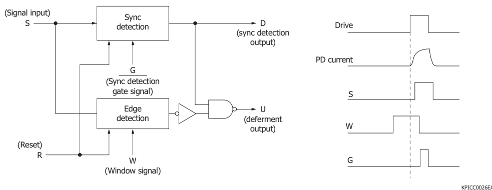
[Figure 4-2] Discrimination circuit block diagram
