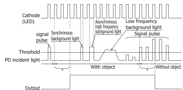
[Figure 1-2] Timing chart
