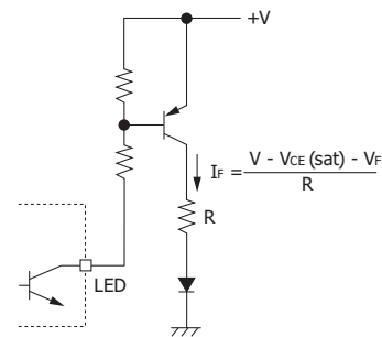
[Figure 5-1] LED drive current enhancing method
