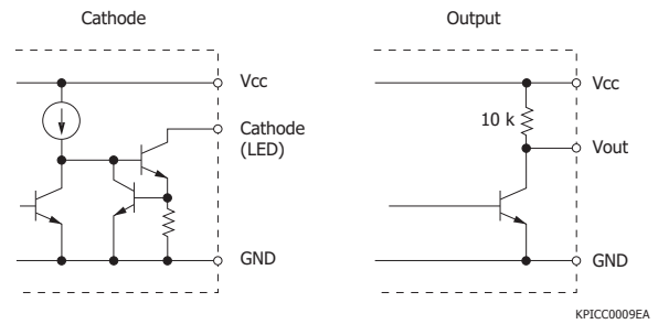
[Figure 2 -1] Output terminal diagram
