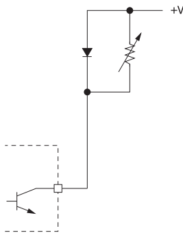
[Figure 5-3] LED drive current adjusting method
