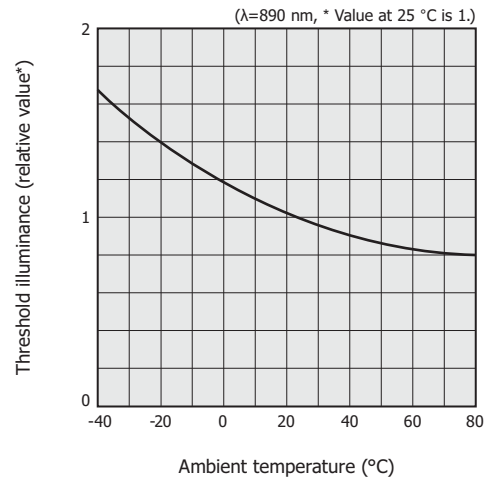
[Figure 3-2] Sensitivity temperature characteristics (typical example)
