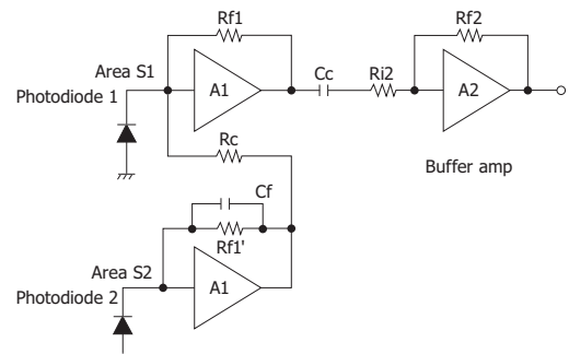
[Figure 2-2] Preamp block diagram
