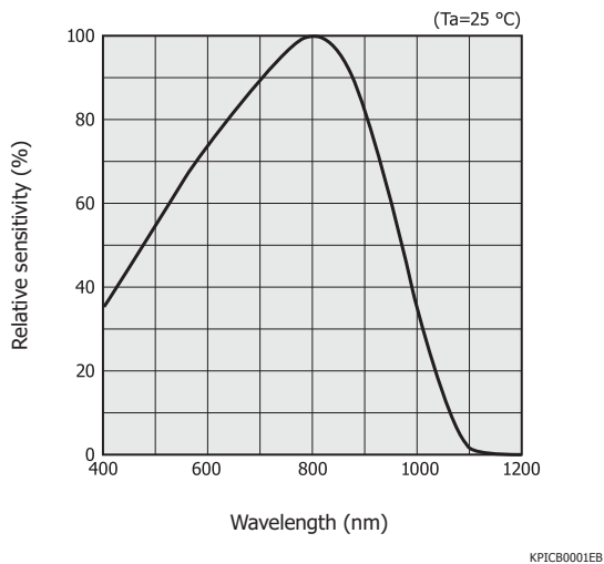
[Figure 3-1] Spectral response (typical example)
