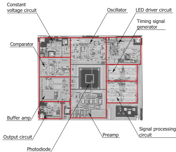
[Figure 1-3] Enlarged photo of chip and block layout
