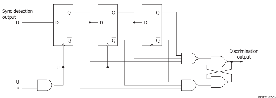
[Figure 4-2] Discrimination circuit block diagram
