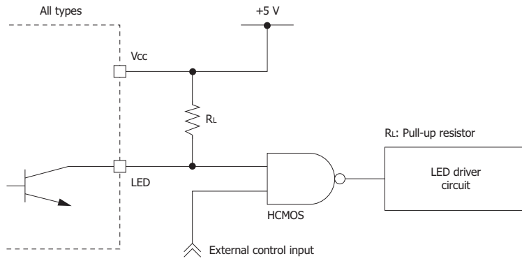
[Figure 5-2] Conversion to logic signal
