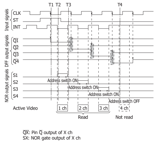
[Figure 6] Shift register operation
