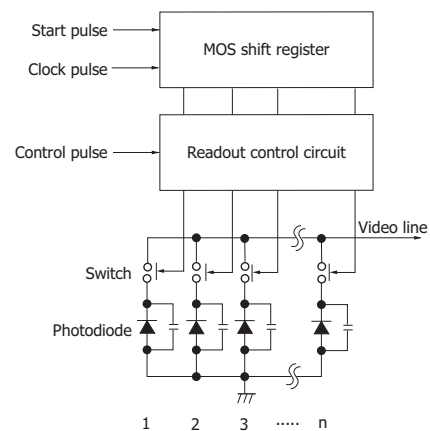
(b) CMOS linear image sensor [S10121 to S10124 series (-01)]
