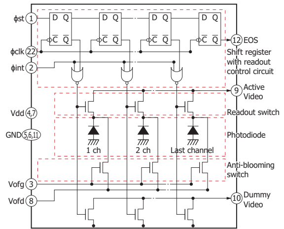
(b) Equivalent circuit
