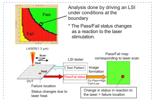
Concept of the analysis of a failed device by utilizing the "drive voltage – operating frequency" characteristics
